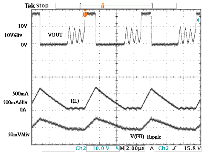
Fig.10 FB Pin Ripple(DCM)
