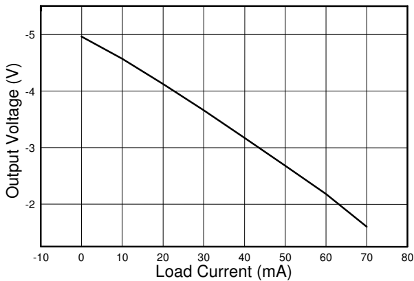
Fig. 3 Output Voltage vs. Load Current (VIN=5V)
