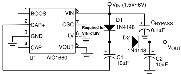
Fig. 10 Voltage Doubling
