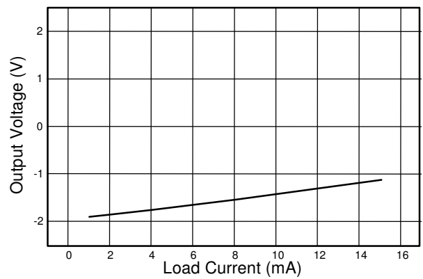
Fig. 4 Output Voltage vs. Load Current (VIN=2V)
