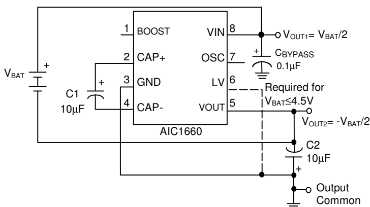
Fig. 12 Battery Splitter
