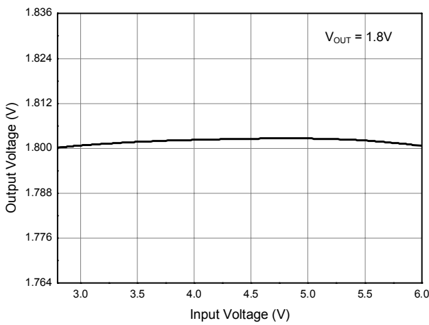
Fig.11 Output Voltage vs. Input Voltage (Vout=1.8V)
