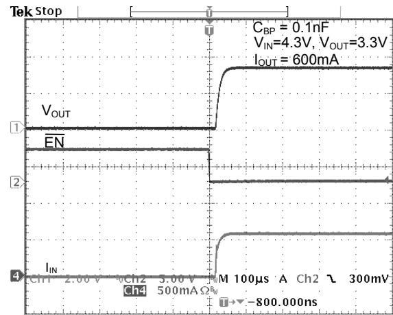
Fig.22 Start-up waveform with 0.1nF bypass capacitor
