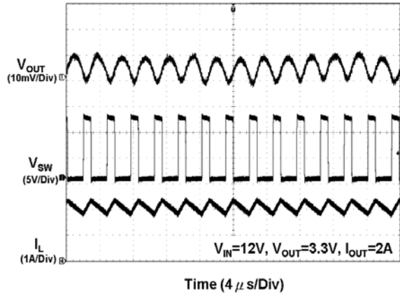
Fig. 8 Output Ripple Voltage
