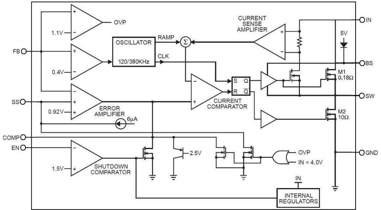
Functional Block Diagram of AIC2562
