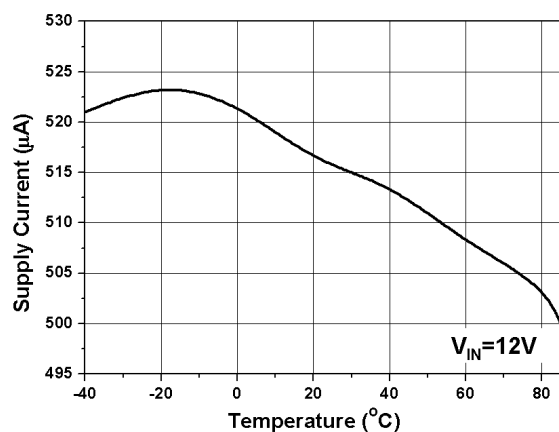
Fig. 6 Supply Current vs. Temperature
