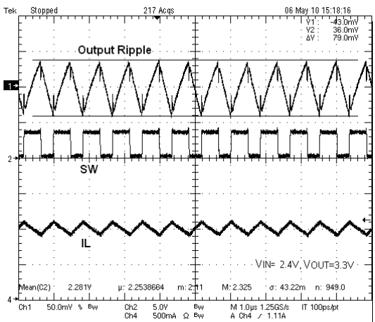
Fig. 17 CCM Switching Waveform at I_{OUT}=550mA
