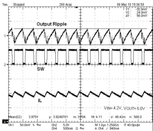
Fig. 18 CCM Switching Waveform at I_{OUT}=700mA
