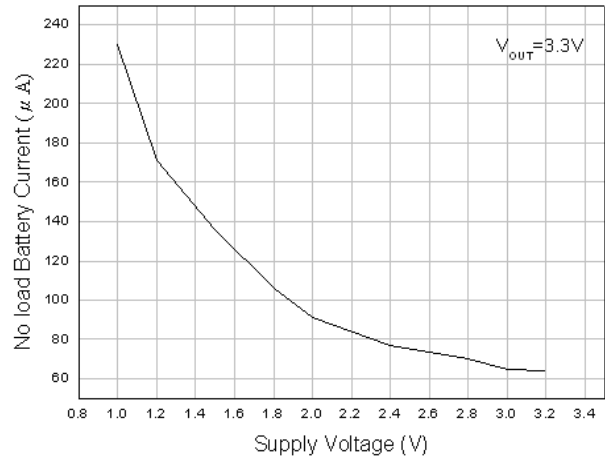
Fig. 4 No load Battery Current vs. Supply Voltage
