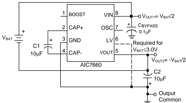
Fig. 18 Battery Splitter
