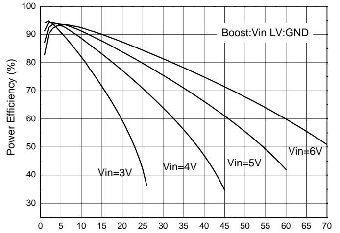
Fig. 6 Power Efficiency vs. Load Current
