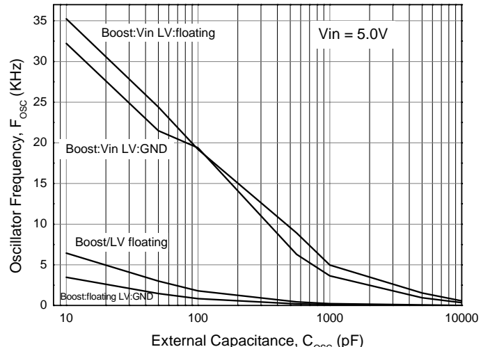
Fig. 10 Oscillator Frequency vs. External Capacitor
