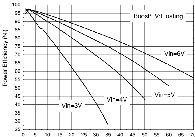
Fig. 5 Power Efficiency vs. Load Current
