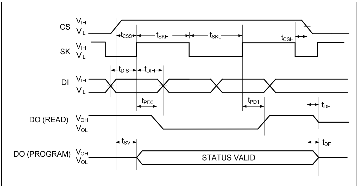
Figure 9 BUS Timing
