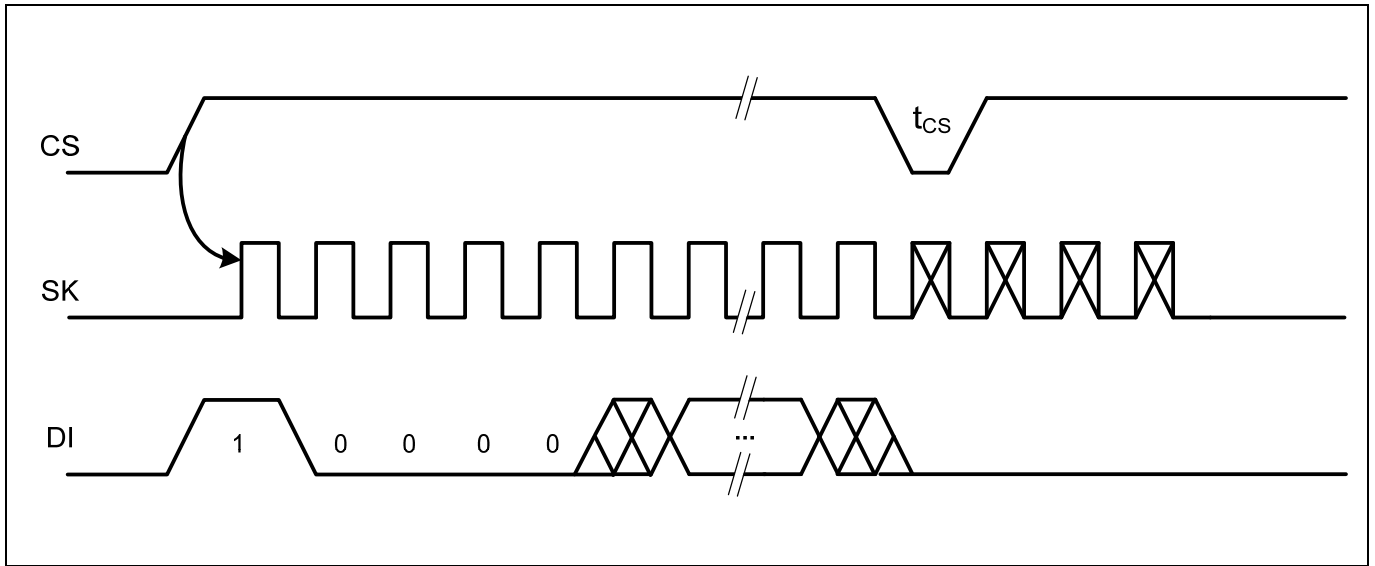
Figure 9 BUS Timing
