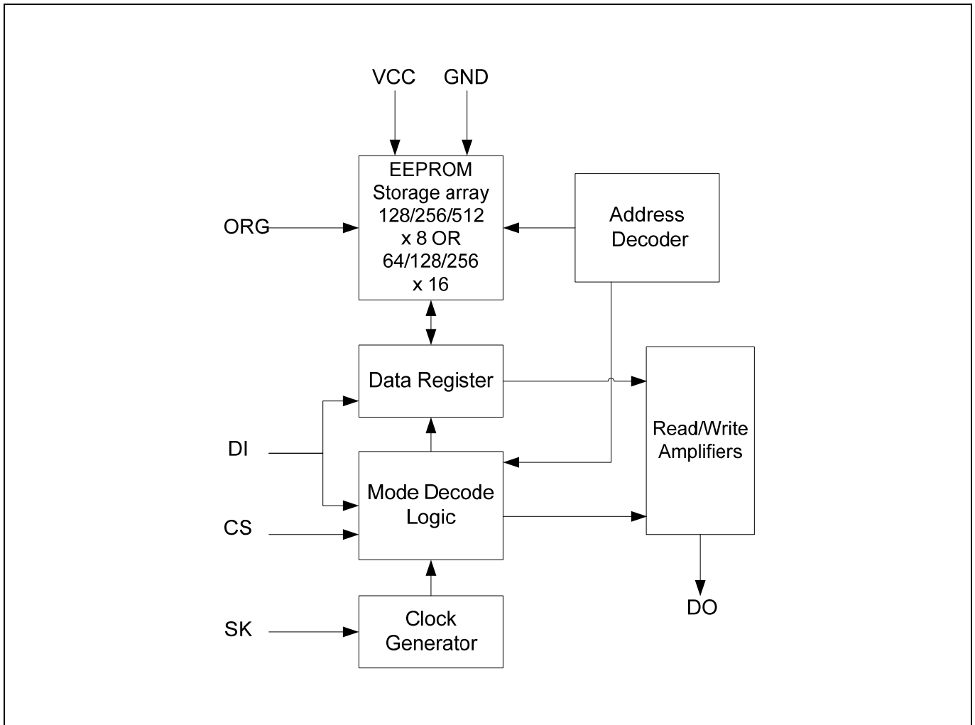
Figure 1 Block Diagram
