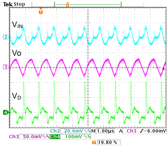
Fig8: 120mA load at Vin=4.2V
